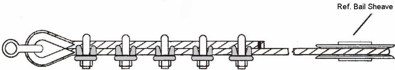
Figure 1: Pendant Cable with Clipped Ends (Old Style)
