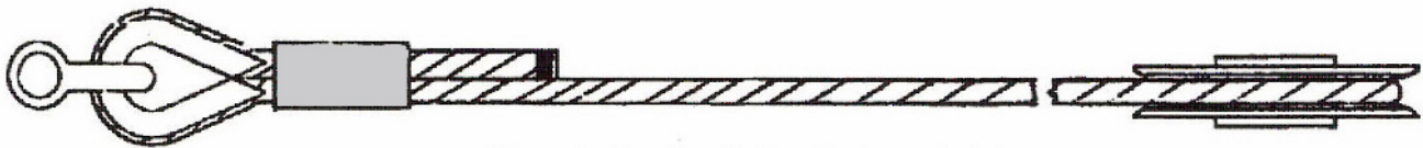
Figure 2: Pendant Cable with Swaged Ends (New Style)
